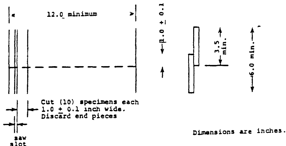
FIGURE 1. Bond strength specimens.
