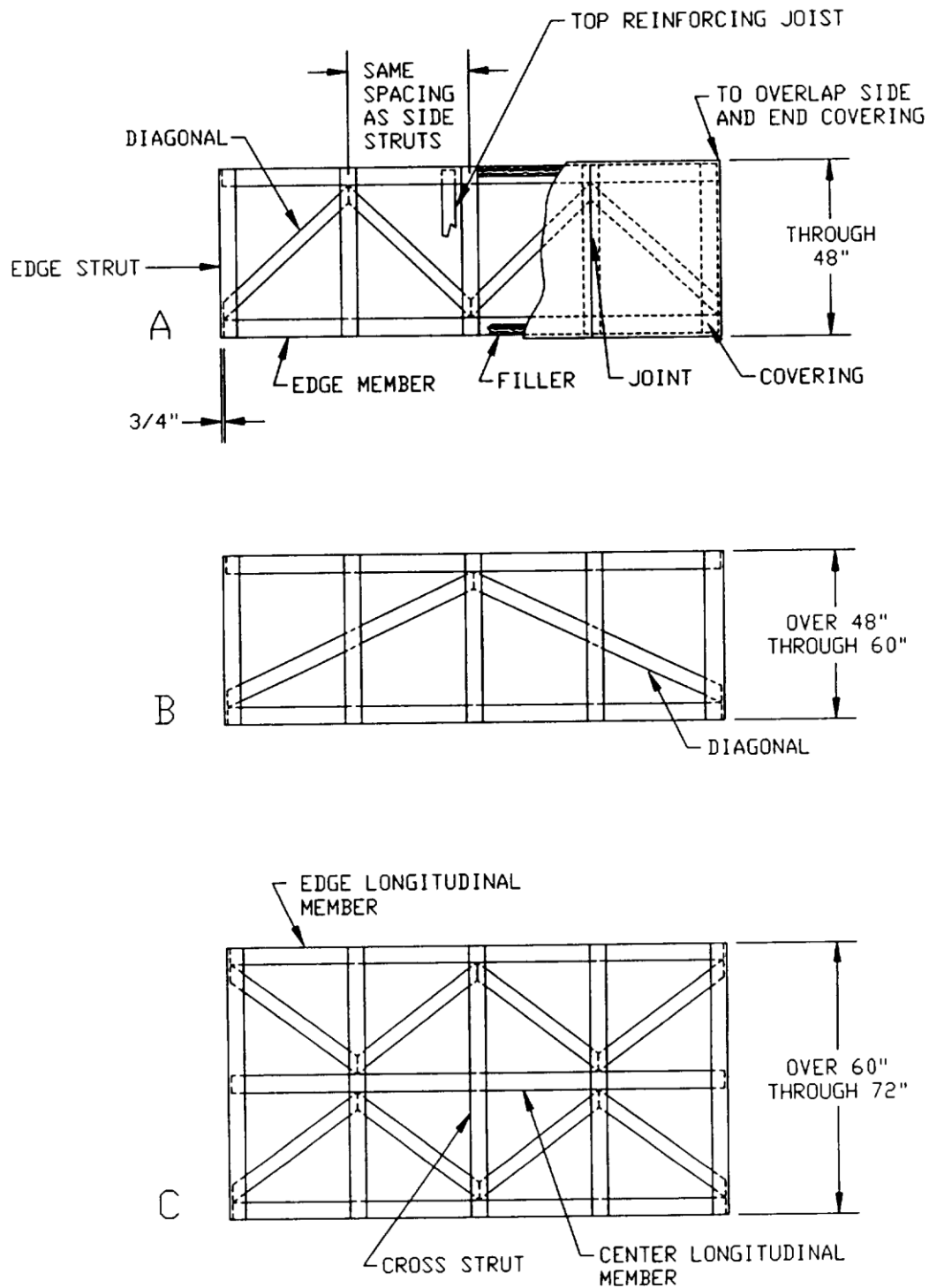
FIGURE 16. Tops for type V, style B crates: A, narrow top; B, medium - wide top; C, wide top.
