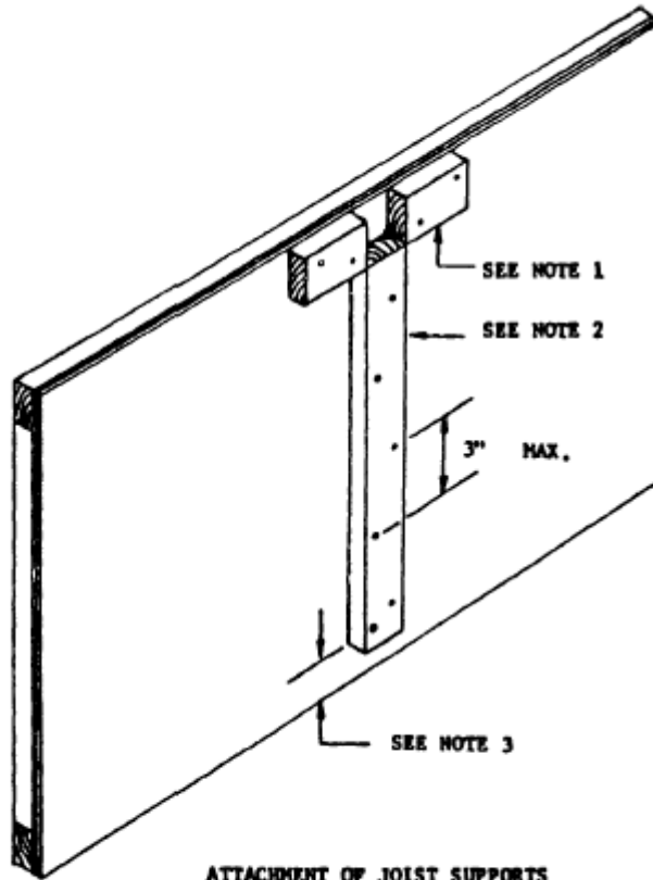
ATTACHMENT OF JOIST SUPPORTS FIGURE 7.
