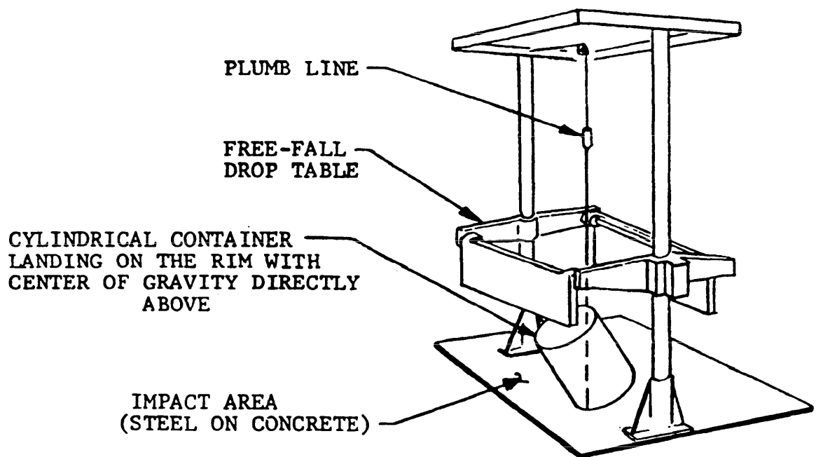
Figure 1. Free-fall drop test.
