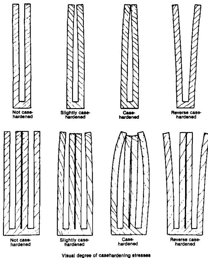
Figure 6-4—Method of cutting stress sections for casehardening tests. Lumber that is less than 1-1/2 in thick is cut into three prongs, and the middle prong is removed; lumber that is 1-1/2 in thick or thicker is cut into six prongs, and the second and fifth prongs are removed. (ML88 5585)
